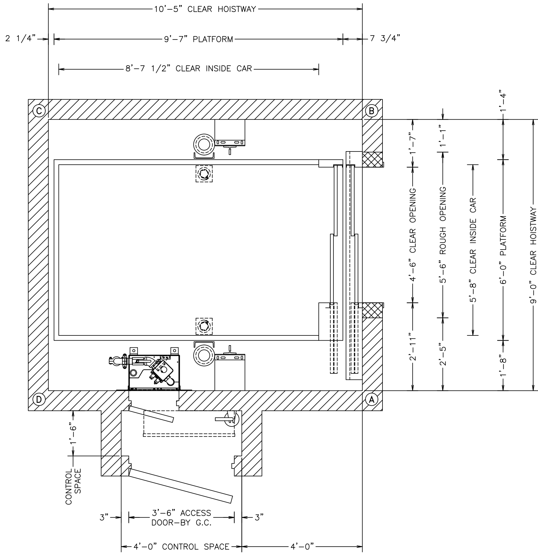
Plan View @ Lowest Landing SCALE : NONE (DEPICTING FEATURES AT VARIOUS LEVELS)
