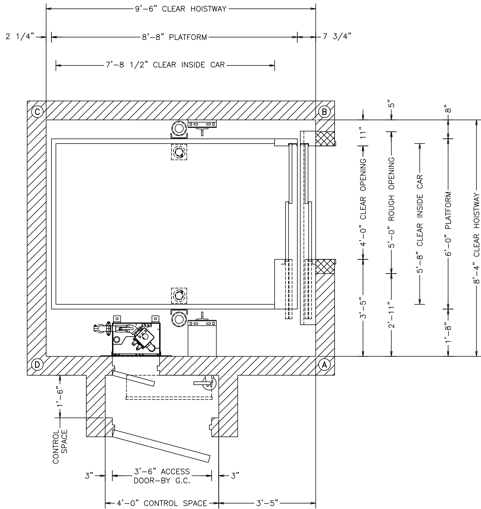
Plan View @ Lowest Landing
