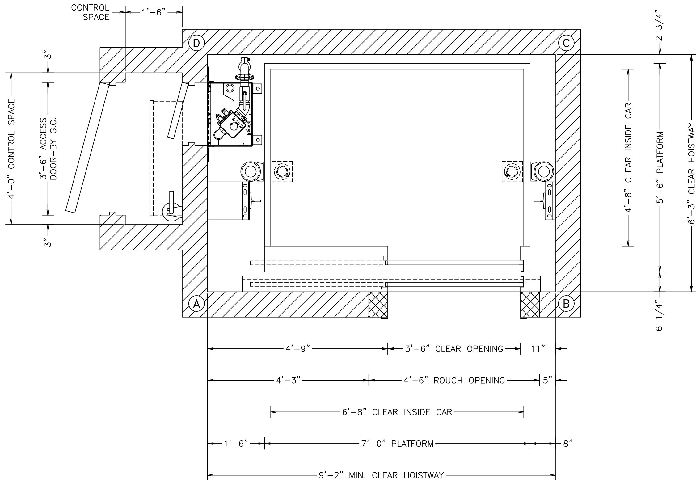
Plan View @ Lowest Landing
