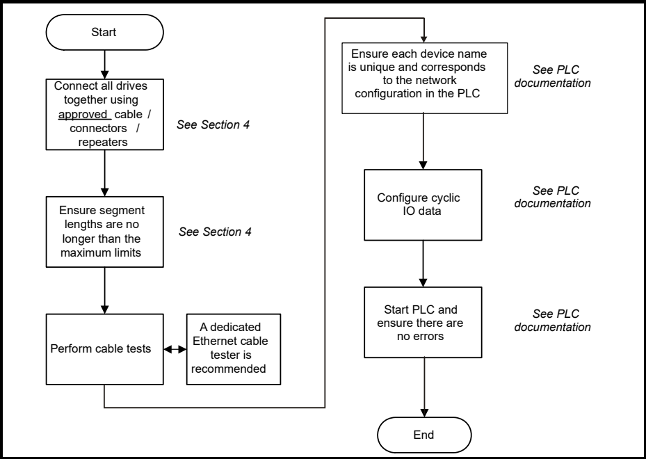
Figure 5-2 SI-PROFINET SR setup flowchart
