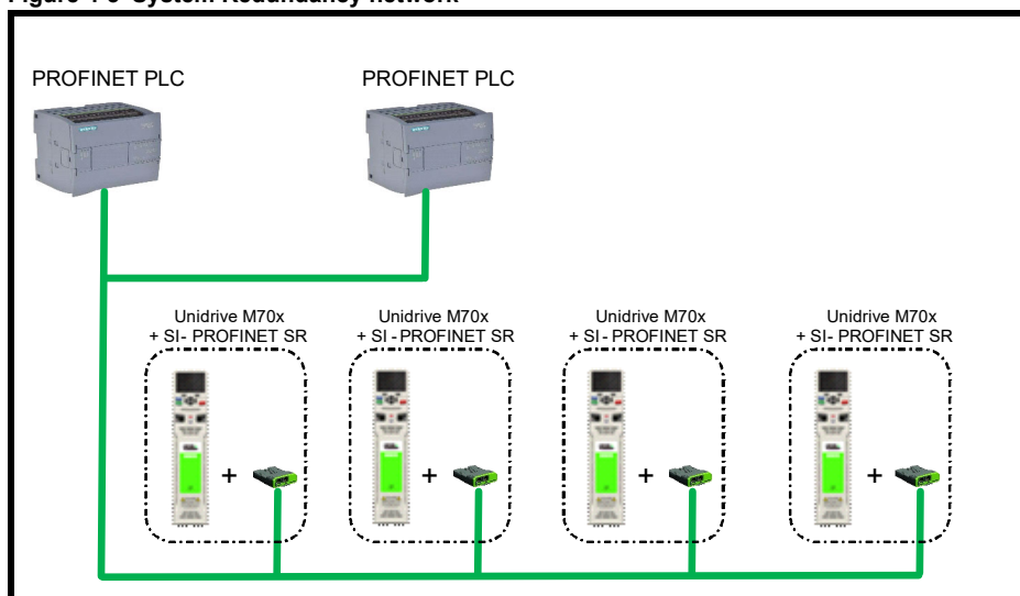
Figure 4-3 System Redundancy network
