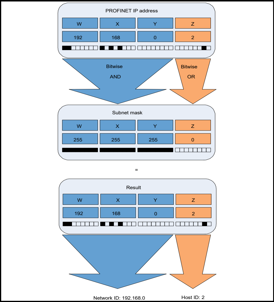
Figure 5-1 Network and host ID
