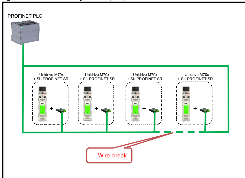
Figure 4-4 Media Redundancy Protocol (MRP) network
