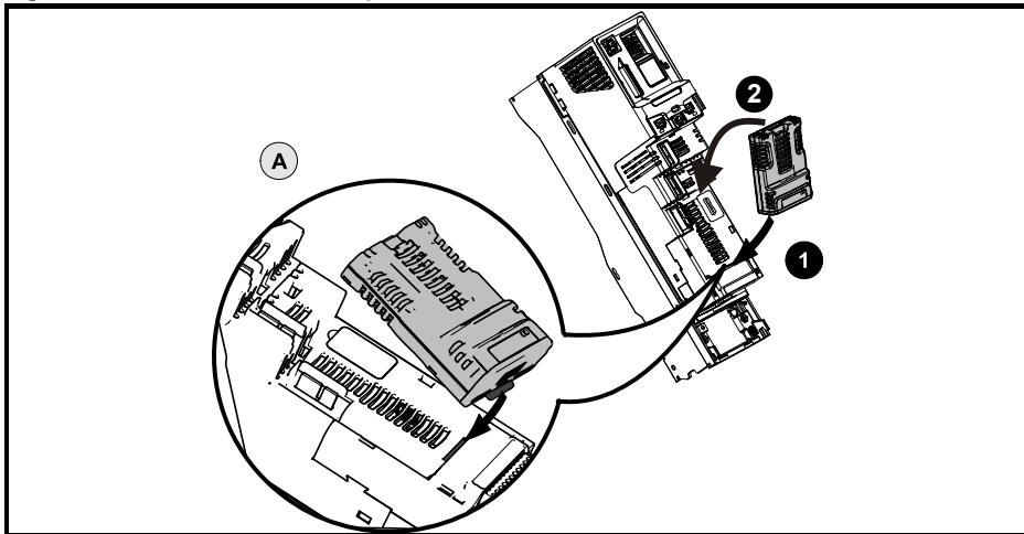
Figure 3-1 Installation of an SI option module on Unidrive M70x
