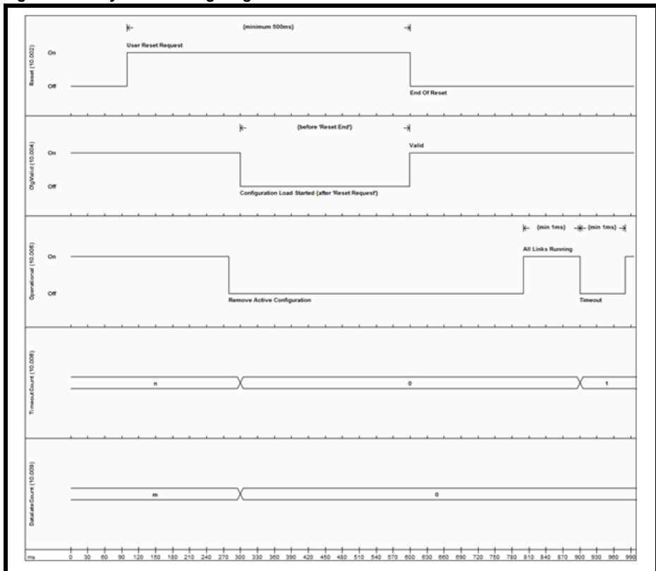
Figure 7-1 Easy Mode Timing Diagram
