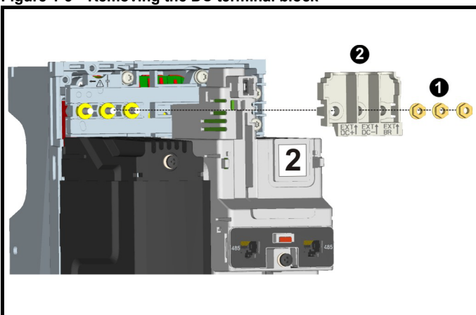
Figure 1-3 Removing the DC terminal block
