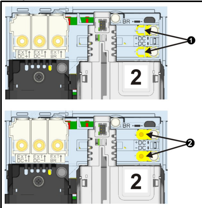
Figure 1-5 Installing the DC - busbar
