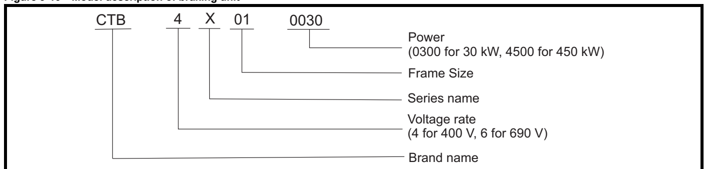
Figure 9-10 Model description of braking unit
