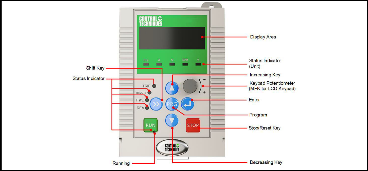
Figure 5-1 Keypad diagram
