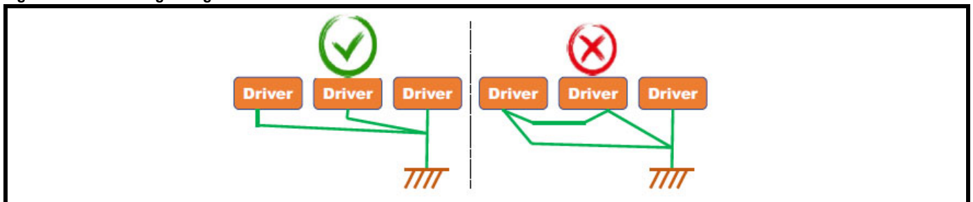
Figure 3-1 Grounding wiring
