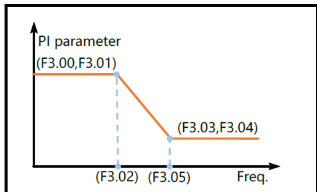
Figure 6-8 Schematic diagram of speed loop PI parameter
