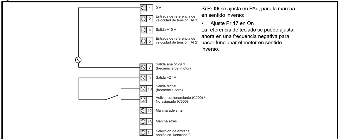
Figura 6-7 Pr 05 = PAd
