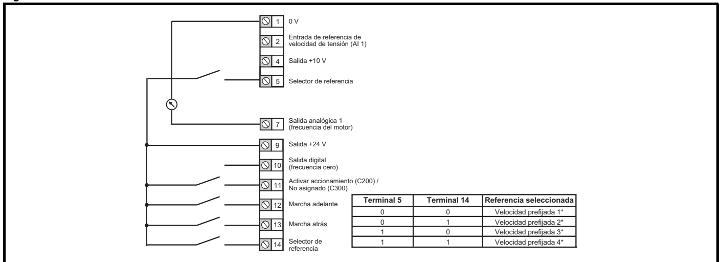
Figura 6-6 Pr 05 = PrESet
