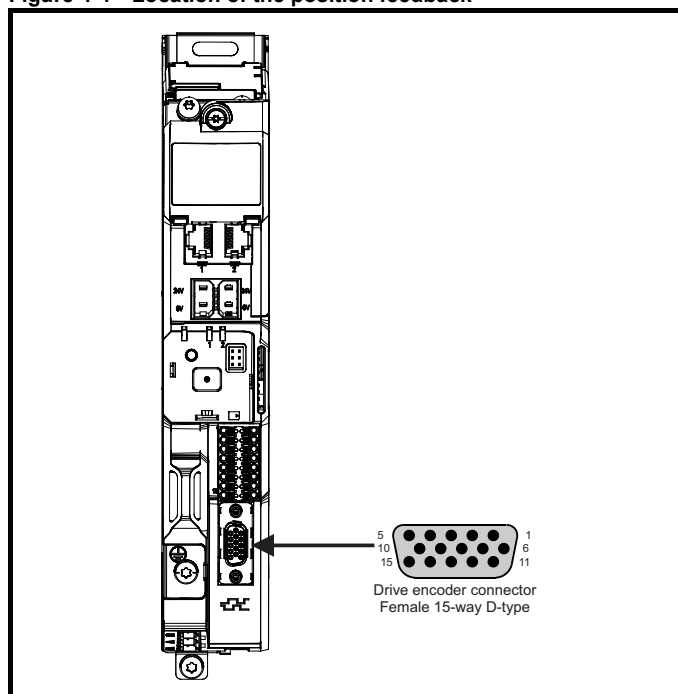
Figure 4-4 Location of the position feedback
